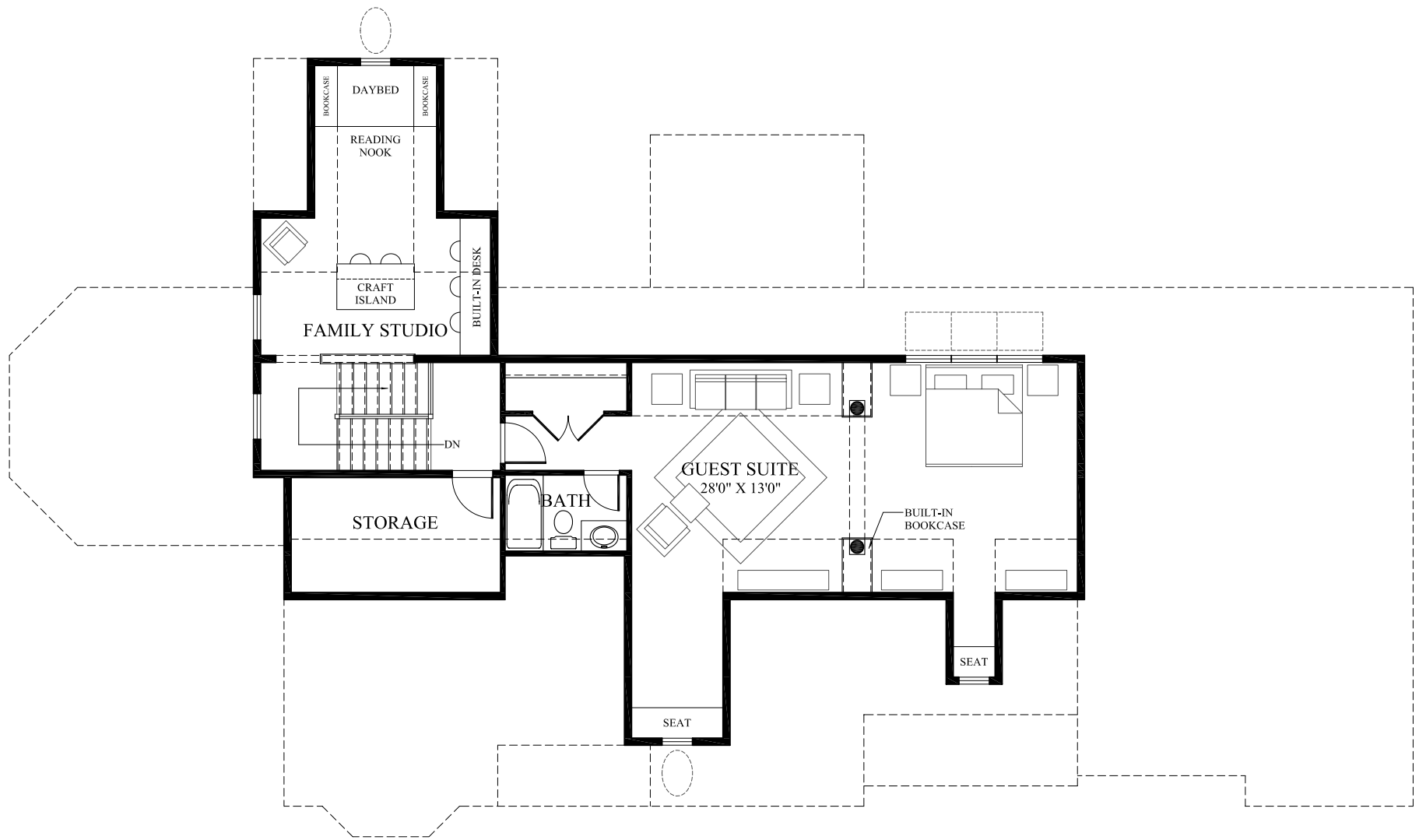
OPTIONAL ATTIC FLOOR PLAN
